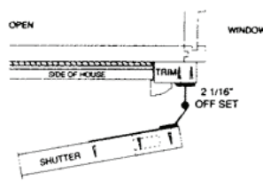
Frame construction
