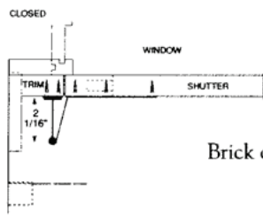
Frame construction
