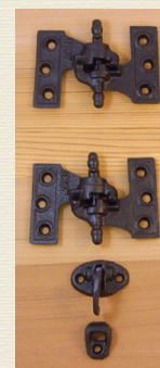
15. ACME Hinge with Gravity Cam
