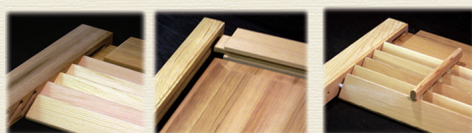
Mortise & Tenon construction enhances the strength and durability of your shutters. (L-R: fixed true louver, raised panel, movable louver)
