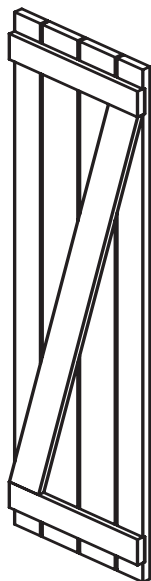
4 Vertical Boards and 2 Horizontal Battens with Single Z-Board
